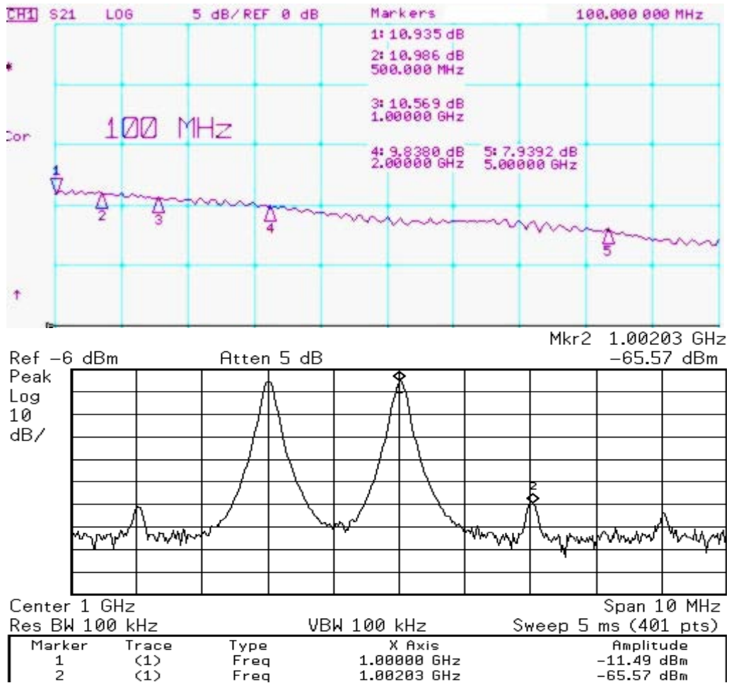
Figure 3. Experimental integrated circuits in linearization research (sponsored by MixSig Labs, Inc., and National Science Foundation). Upper left is layout of 0.18- \mu\text{m} CMOS, linearized RF integrated circuit; upper right is simplified block diagram of patented linearization method; middle is measured gain up to 5 GHz; bottom is two-tone linearized spectrum measured at 1 GHz. (Led by faculty member Dr. Tom Weldon).
